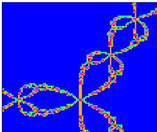
図3 julia
